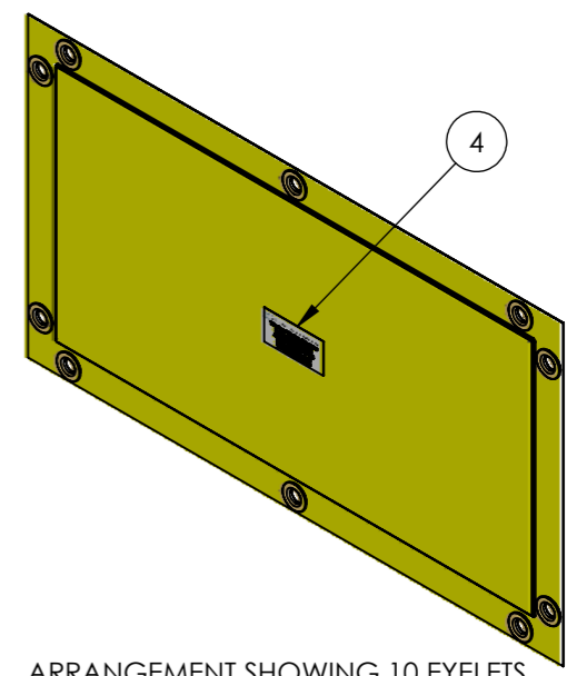
ARRANGEMENT SHOWING 10 EYELETS
